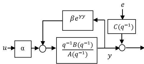
Figure 3: Model of the system
