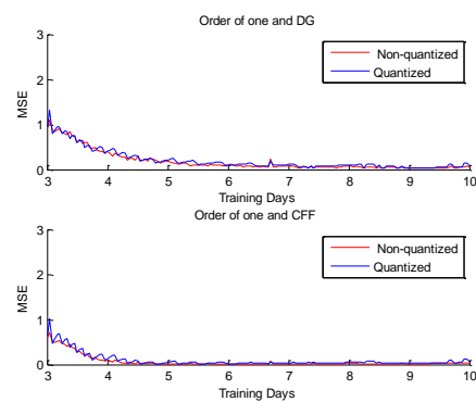
Figure 7: ARX of order one in the presence of organic heat.
