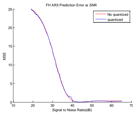
Figure 12: Noise Robustness for FH method
