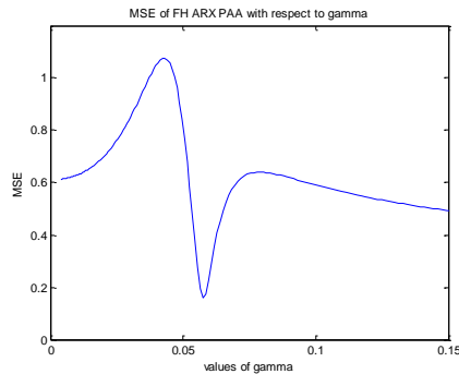
Figure 6: Prediction accuracy vs. \gamma
