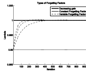
Figure 4: Types of forgetting factors.
