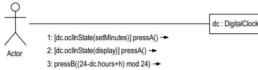
Figure 5. A collaboration diagram realizing the use case setHours(h : Integer)
